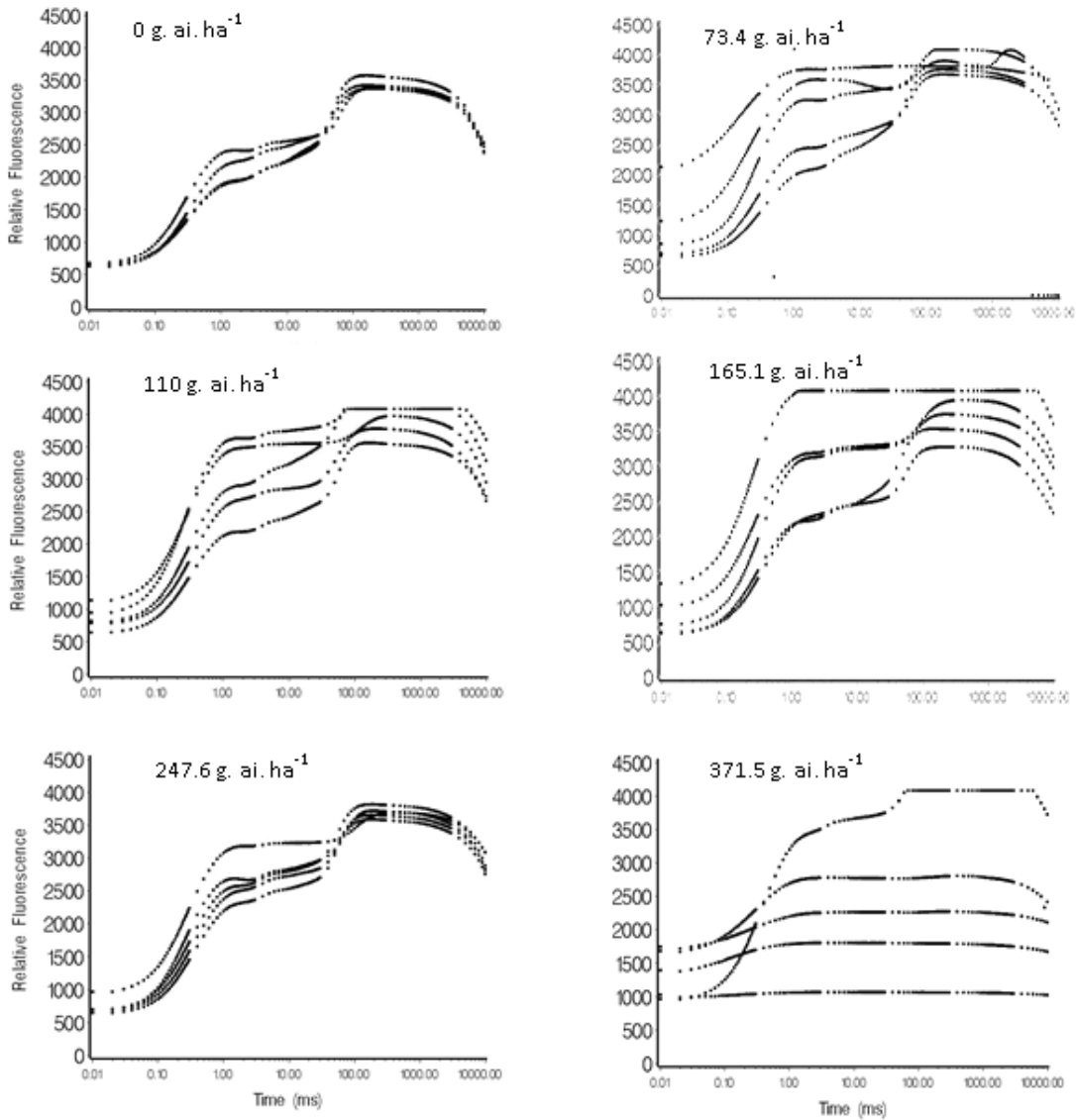
Fig 2. Effect of different doses of dicamba+2, 4-D on the shape of the Kautsky curves (10 s) at S. arvensis 2 days after spraying. Each curve presenting one replication. Changes at the shape of the Kautsky curve compare to the standard shape of healthy S.arvensis (0 g. ai. ha -1 ) shows that PSII is damaged.
