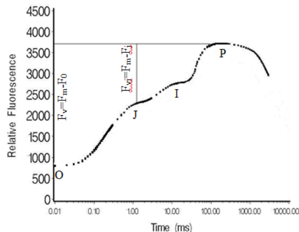
Fig 1. Kautsky curve recorded with Handy PEA instrument in a 30 minutes dark adapted leaf. The Kautsky curve rise from O to P levels is characterized by the OJIP steps reflecting PSII electron transport from water to PQ pool.
