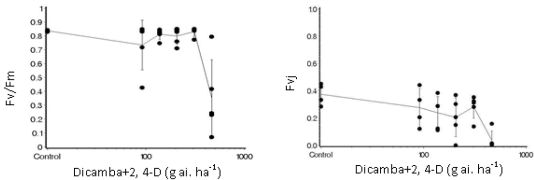
Fig 3. Effect of dicamba+2, 4-D doses on chlorophyll fluorescence parameters at 2 days after spraying. Each point presenting one replication. Decreasing of these two parameters shows that plants photosynthesis is not working properly.
